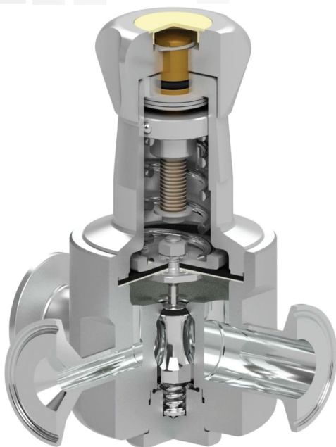
Cut away view with pressure gauge connection
